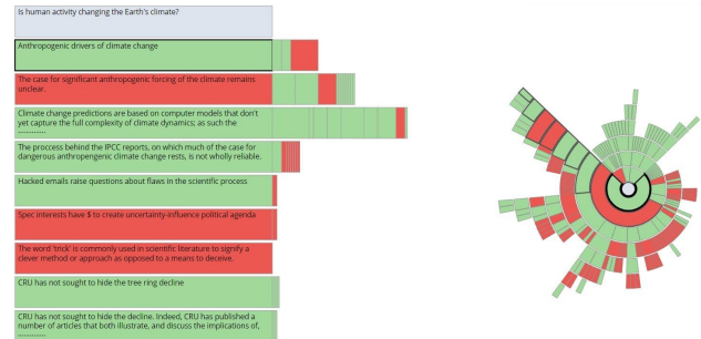
Figure 7: Stacked Boxes on the left for reading the text with coordinated sunburst overview on the right for navigating the structure.
