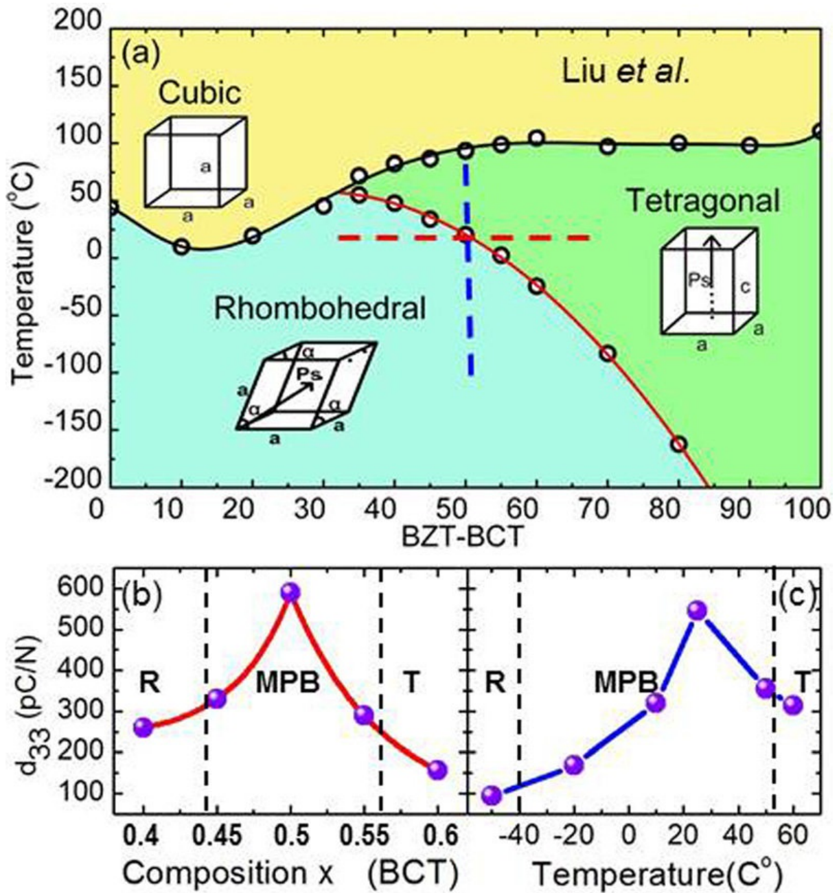
Figure 5. (a) \text{Ba}(\text{Ti}_{0.8}\text{Zr}_{0.2})\text{O}_3-x(\text{Ba}_{0.7}\text{Ca}_{0.3})\text{TiO}_3 ceramic phase diagram near the MPB; (b) composition-dependence of d_{33} during composition-induced R-MPB-T transition along the red horizontal line displayed in (a); (c) temperature-dependence of d_{33} during temperature-induced R-MPB-T transition along the blue vertical line displayed in (a);
