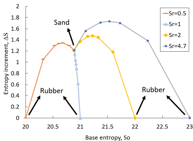
Fig. 2 Grading entropy of RSm with change in size ratio based on Lee et al. (2010)
