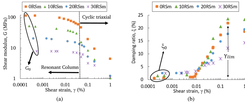
Figure 1. a) Shear modulus and b) damping ratio of RSm from small-to-large strains (Bernal-Sanchez, 2020)
