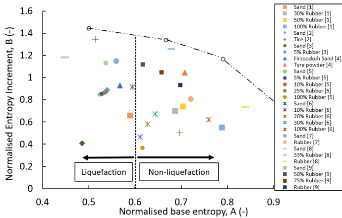
Fig. 9 Stability of RSm based on the literature: [1] = Kaneko et al., 2013; [2] = Otsubo et al., 2016; [3] = Promputthangkoon and Hyde, 2008; [4] = Bahadori and Roohollah, 2018; [5] = Shariatmadari et al., 2018; [6] = Bernal-Sanchez, et al., 2020, [7] = Enquan and Qiong, 2019; [8] = Rios et al., 2021; [9] = Amuthan et al., 2020.
