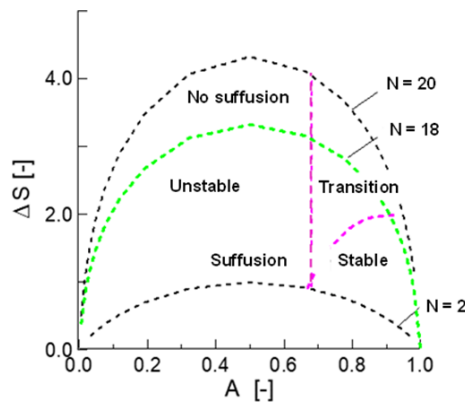
Fig. 7 Internal or grain structure stability criterion in the partly normalized diagram (modified after Lőrincz, 1986).
