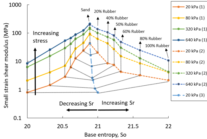
Fig. 5 Change in soil stiffness of RSm with base entropy ( S_o ) and confining pressure at S_r = 0.5 (1), S_r = 2 (2), and S_r = 1 (3) based on Lee et al. (2010)
