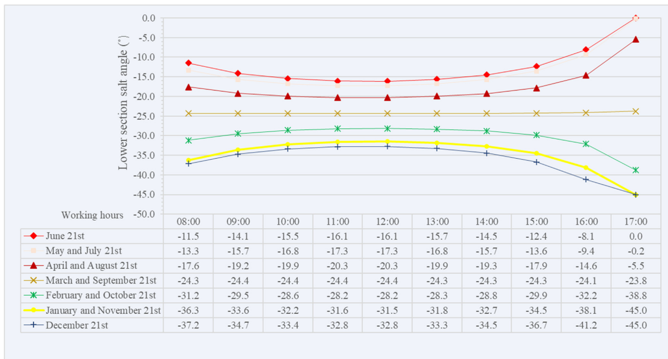
Fig. 9. The proposed scheduled slat angle for the lower section (all slats) of the split louver.
