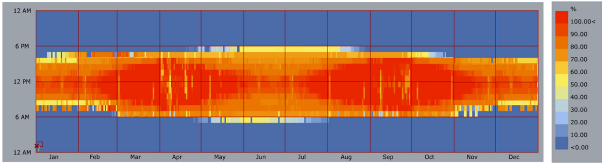
Fig. 17. Annual hourly percentage coverage within UDI_{150-750} lx for the split louver with scheduled slat angle for both upper and lower sections.
