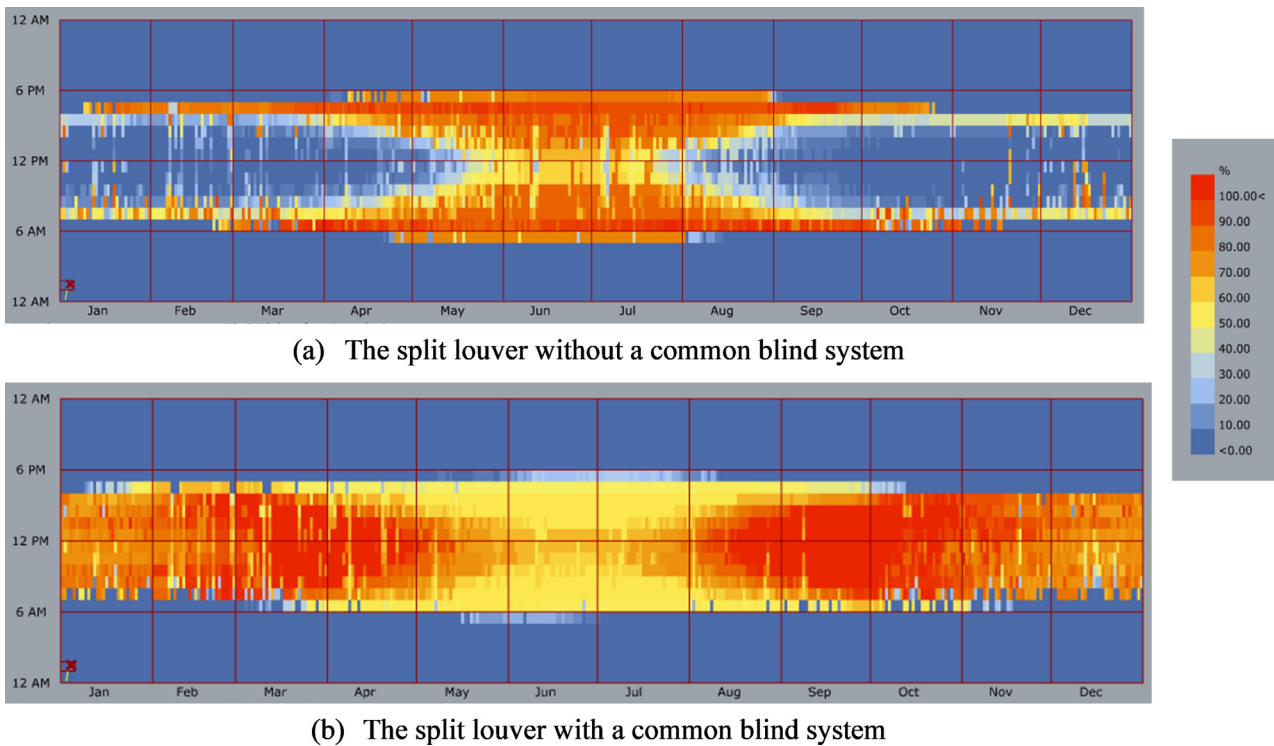
Fig. 11. Annual hourly percentage coverage within UDI 150~750 lx showing the blinds performance in the split louver.
