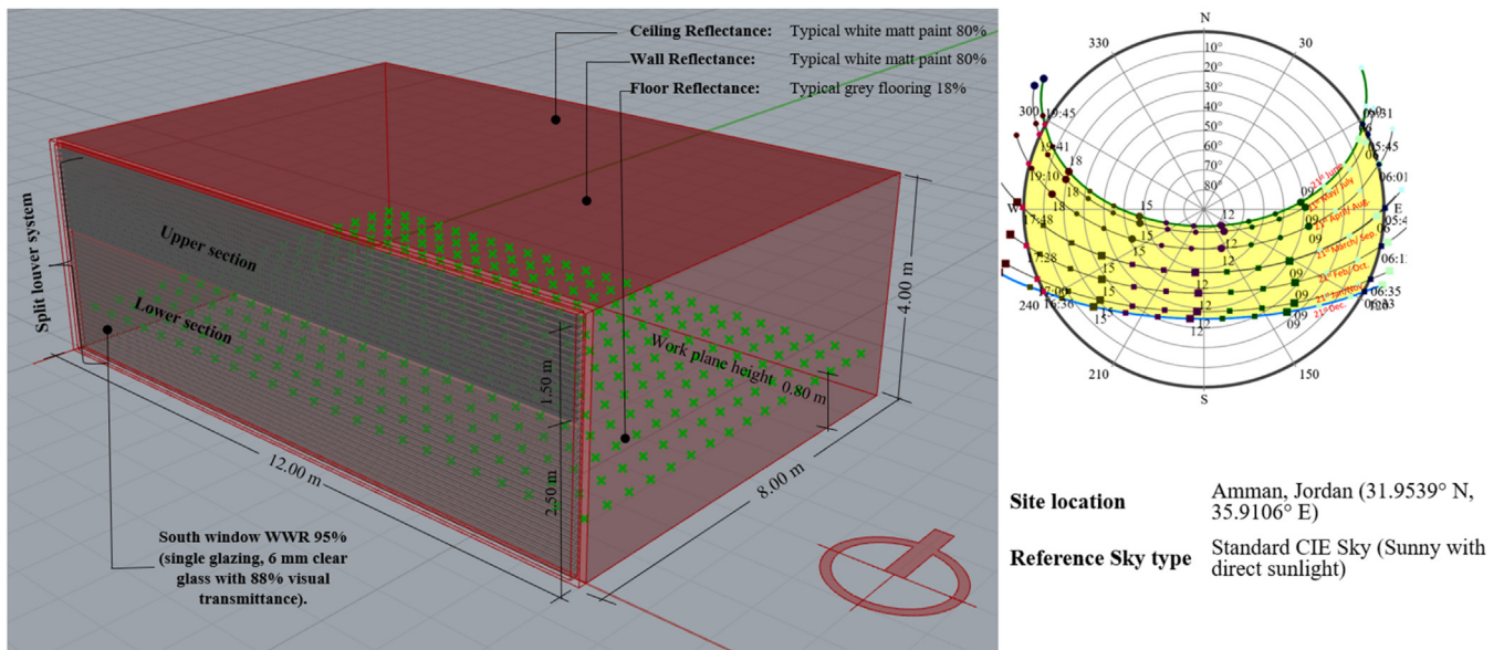
Fig. 3. Base model configuration of a virtual office room.
