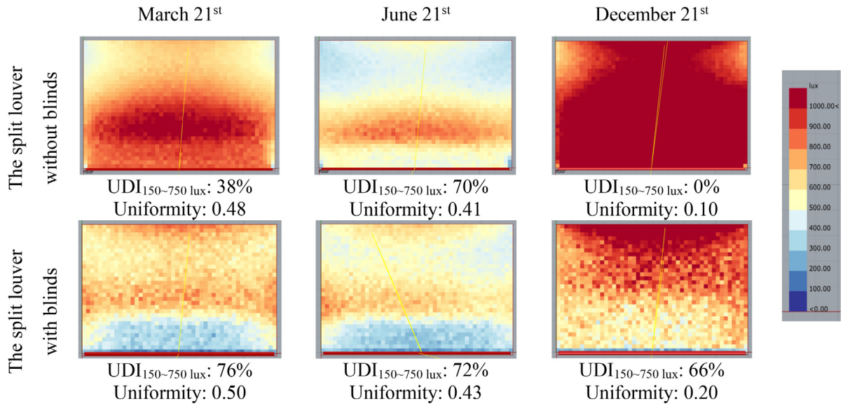
Fig. 10. Illuminance maps for the split louver and blinds system on the three typical days at 12:00 pm.
