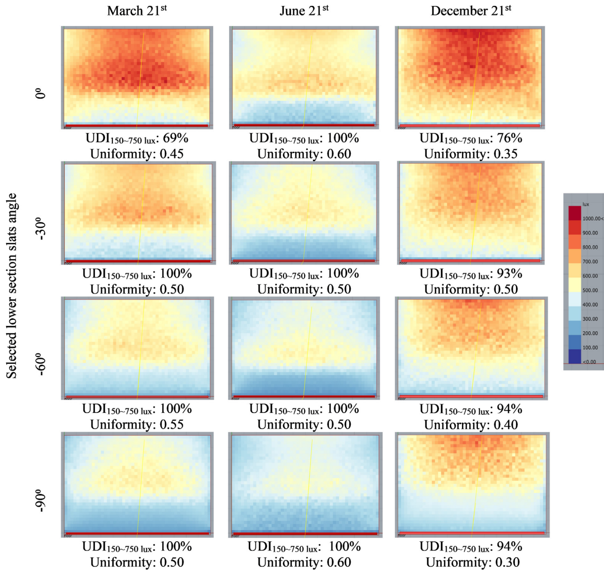
Fig. 14. Illuminance maps for various combinations of different slat angles of the lower section of the split louver and semi-mirrored parametric slat in the upper section on the three typical days at 12:00 pm.
