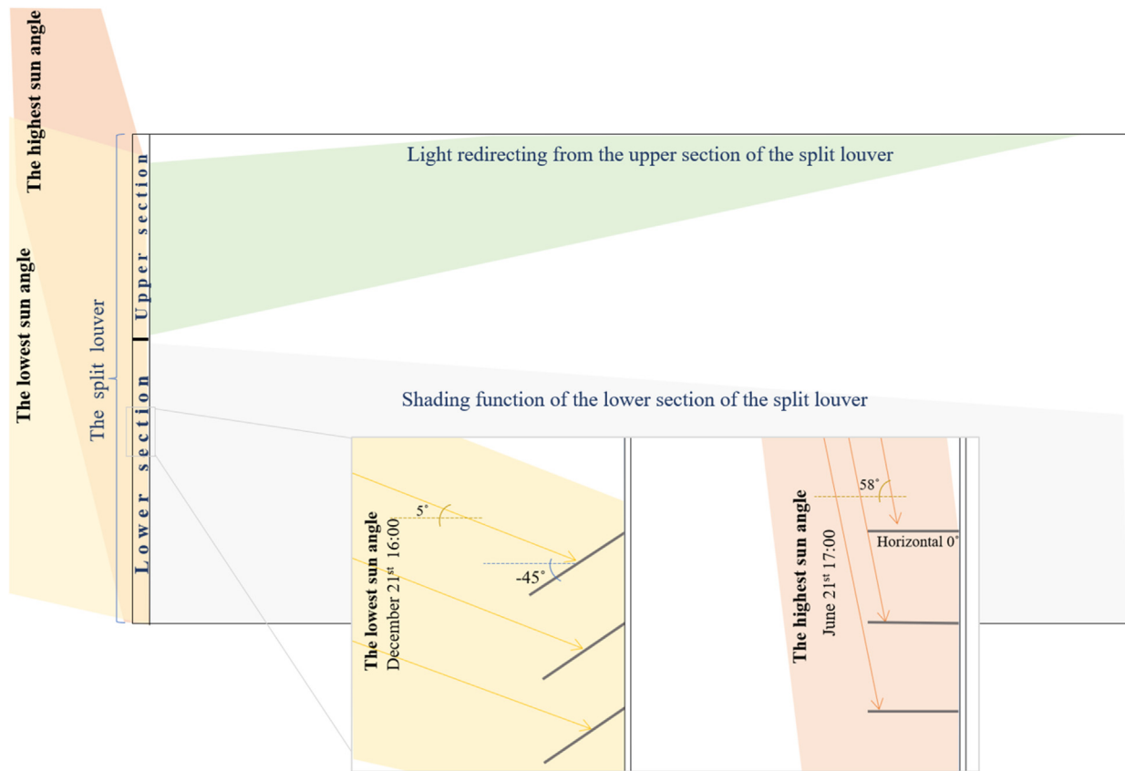
Fig. 8. The slats angle of the lower section responding to the lowest and highest sun angles.
