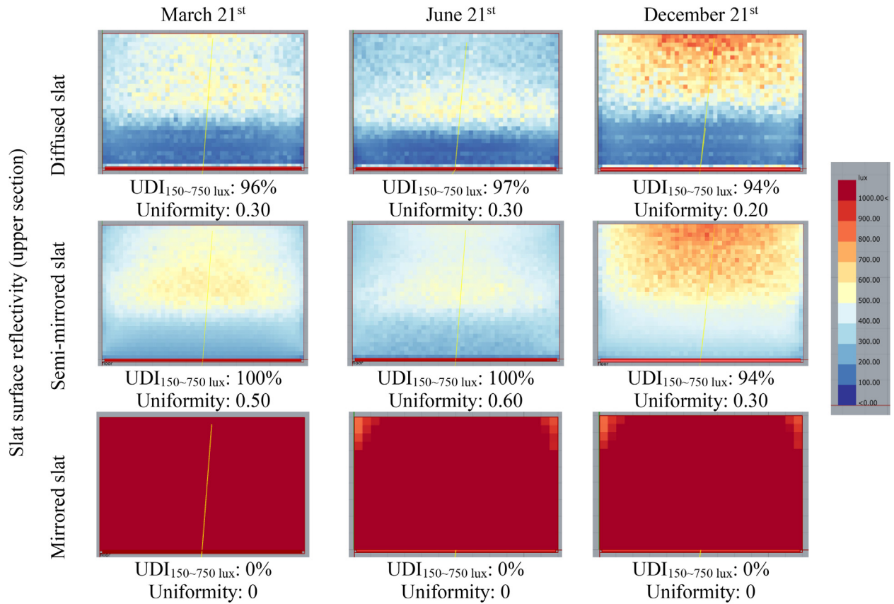
Fig. 12. Illuminance maps for various combinations of the split louver with different slat surface reflective features in the upper section (closed lower section) on three typical days at 12:00 pm.
