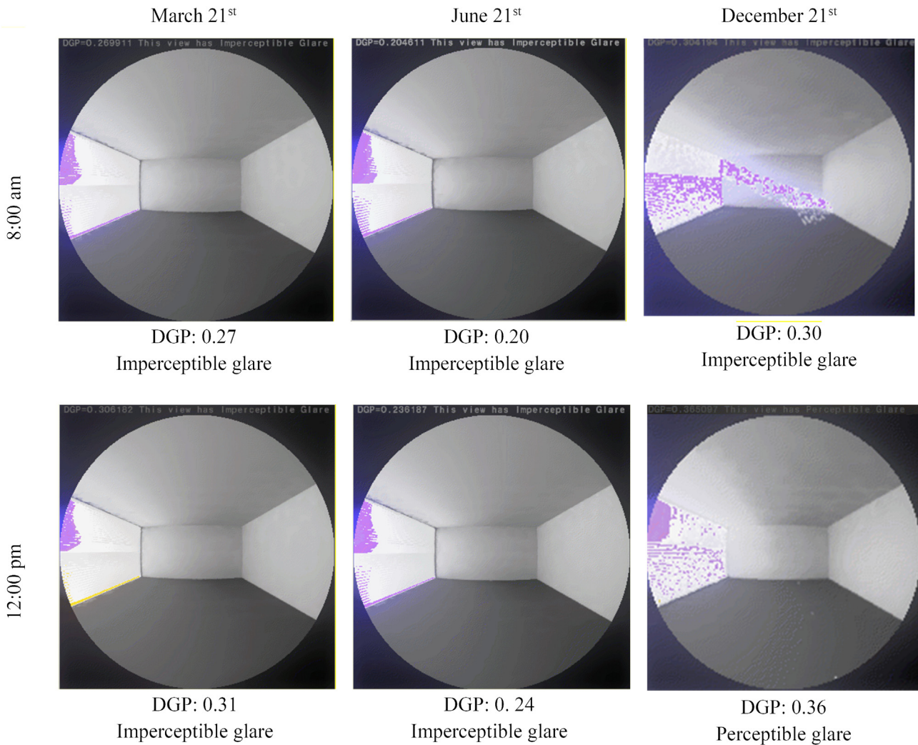
Fig. 18. Daylight glare probability (DGP) of the split louver with scheduled slat angle.
