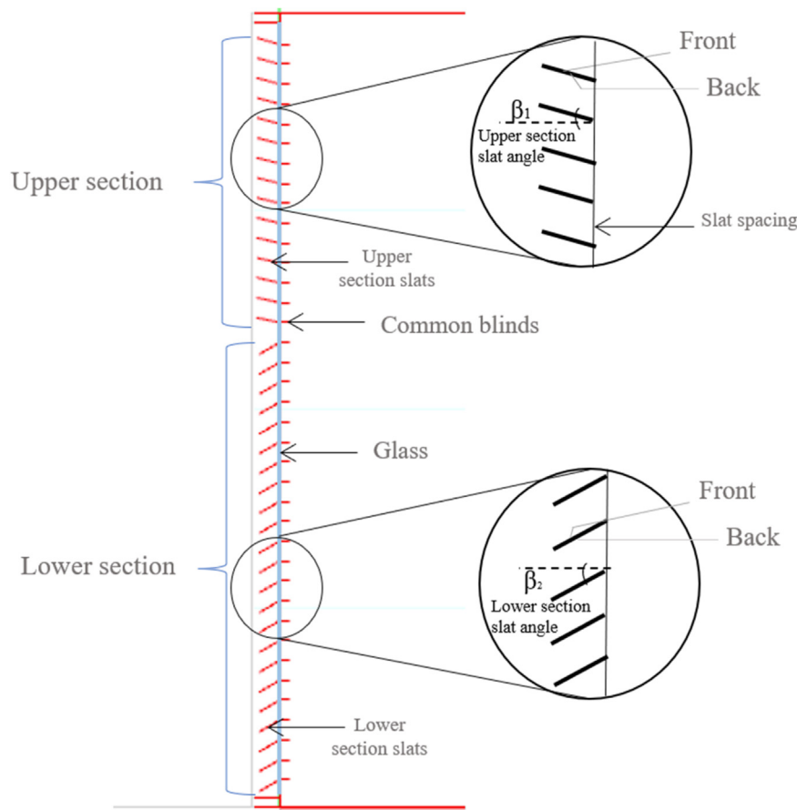
Fig. 4. Split louver design description.
