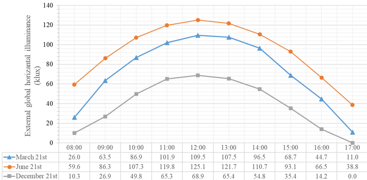
Fig. 2. External global horizontal illuminance (klux) for the working hours on the three typical dates.
