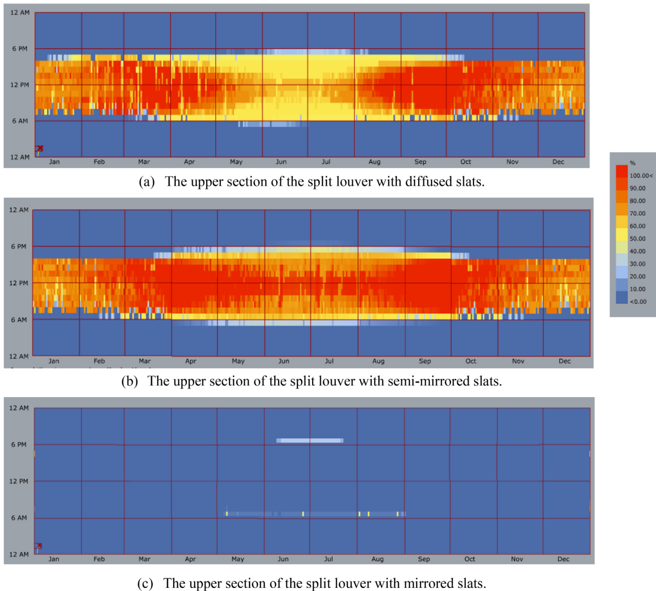
Fig. 13. Annual hourly percentage coverage within UDI 150-750 lx of the split louver with different slat reflective features in the upper section.
