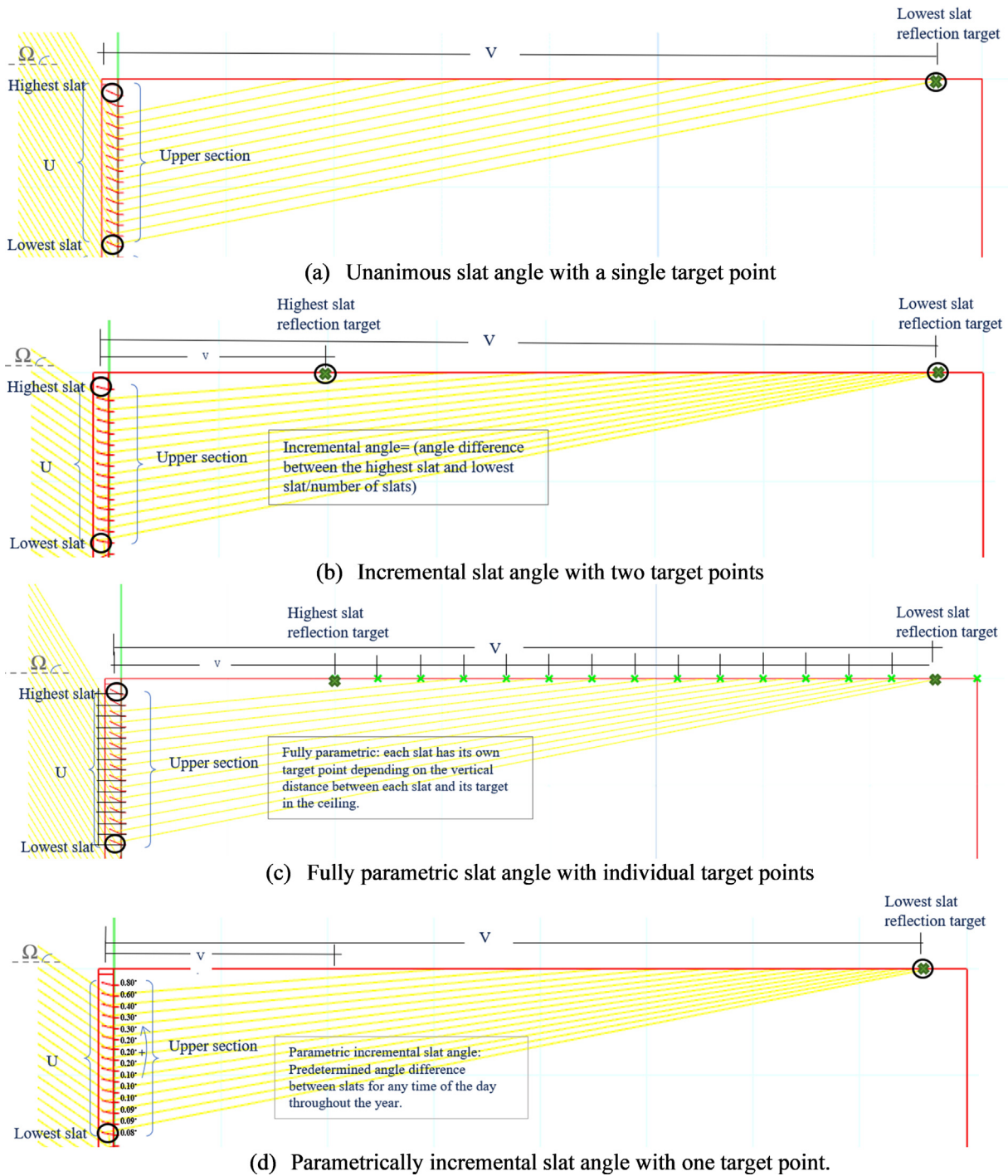
Fig. 5. Different slat angle systems for the upper section of the split louver.
