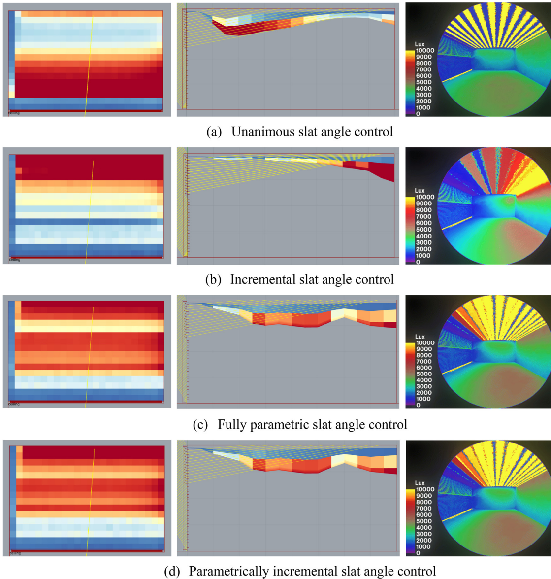
Fig. 6. Comparison of daylighting performance of split louver with different slat angle controls in the upper section and closed lower section on March 21st at 12:00 pm: (a) unanimous, (b) incremental, (c) fully parametric, and (d) parametrically incremental slat angle control.
