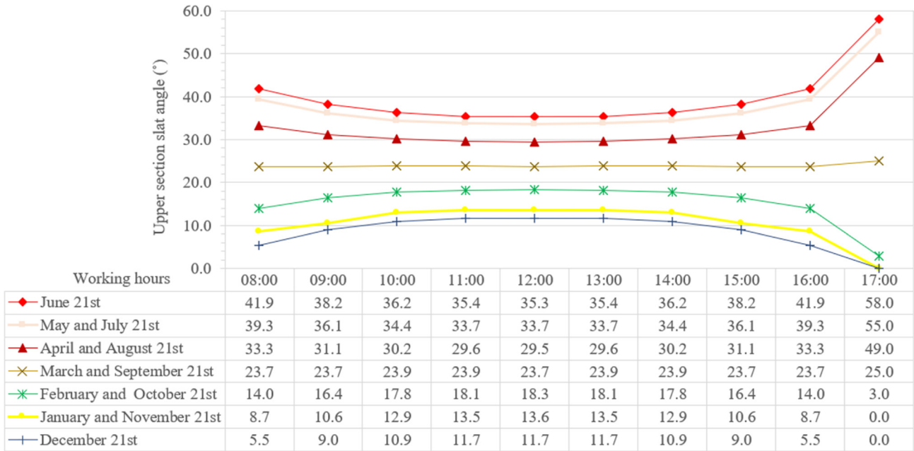
Fig. 7. Parametric tilt angle of the lowest slat in the upper section of the split louver (parametrically incremental control).
