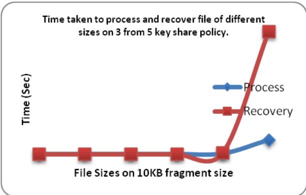
Fig. 9: Process and Recover of file using 10KB fragment size on 3 from 5 Policy.
