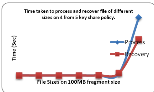
Fig. 13: Process and Recover of a file using 100MB fragment size on 4 from 5 Policy.
