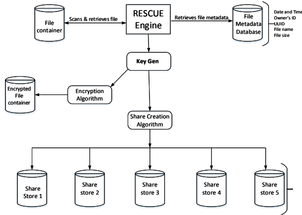
Figure 1: Key/File share creation
