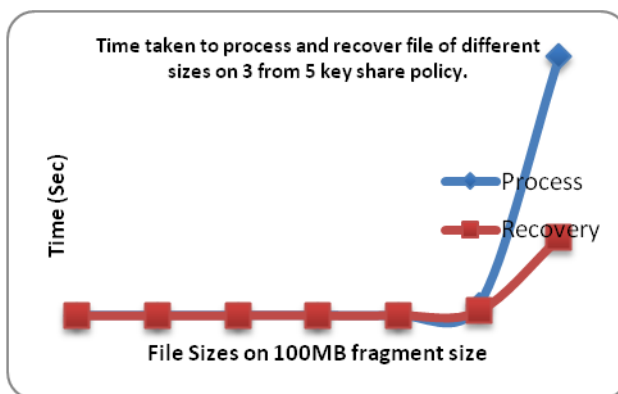
Fig. 12: Process and Recover of a file using 100MB fragment size on 3 from 5 Policy.
