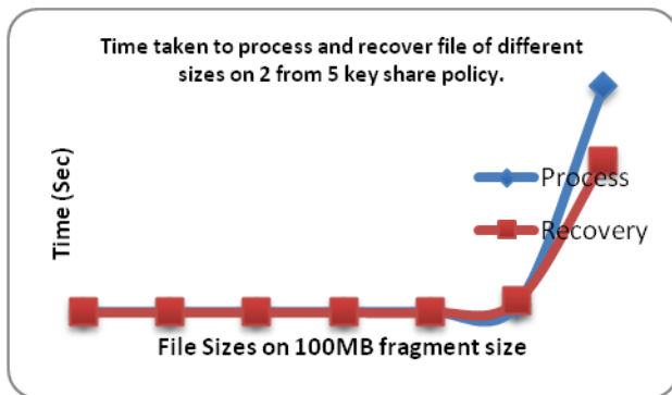
Fig. 11: Process and Recover of file using 100MB fragment size on 2 from 5 Policy.
