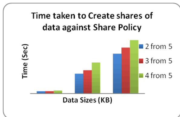
Fig. 4: Time taken to Create share against Policy
