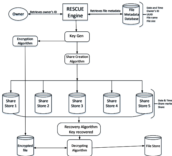
Figure 3: Key recovery and File decryption
