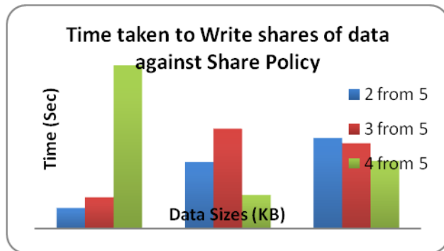
Fig. 5: Share Writing to folders against Policy
