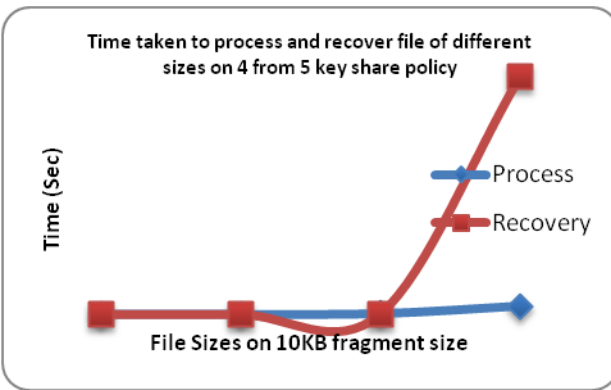
Fig. 10: Process and Recover of file using 10KB fragment size on 4 from 5 Policy.
