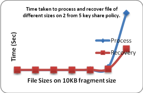
Fig. 8: Process and Recover of file using 10KB fragment size on 2 from 5 Policy.
