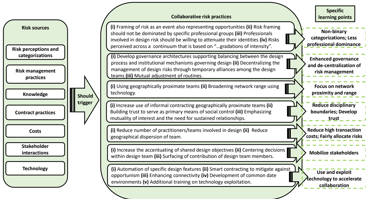
Figure 4: Summary findings
