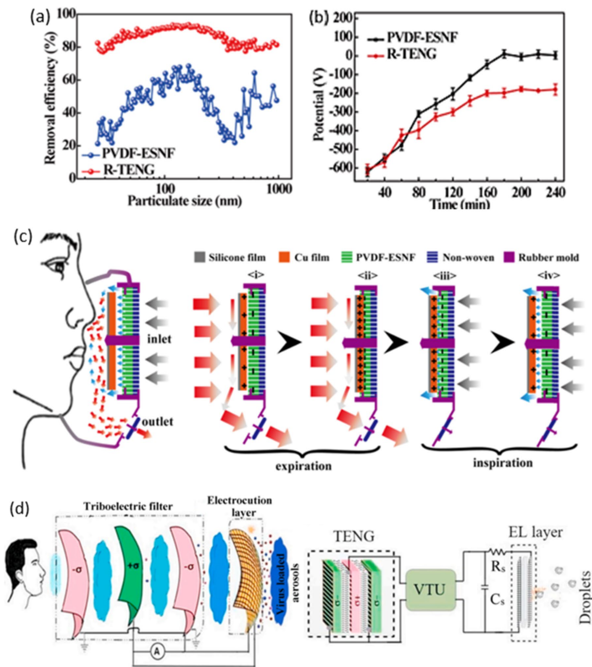
Fig. 16 Self-charged electret air filters by triboelectric nanogenerators: a Corresponding removal efficiency of the PVDF-ESNF and R-TENG. b Average surface potential change of the single PVDF-ESNF and the PVDF-ESNF implanted in the R-TENG in 240-min filtration. c Working principles of R-TENG self-powered face mask by periodic expiration and inspiration (Reproduced with permission from [151], Copyright American Chemical Society, 2018). d Schematic representation of the proposed triboelectric multilayers com-
