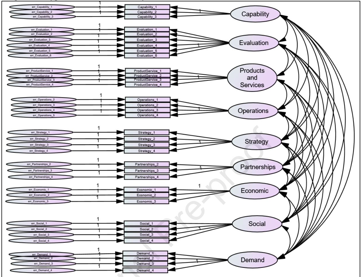
1 Figure C: Hypothesized Confirmatory Factor Structure of the Sustainable Innovation Scale
