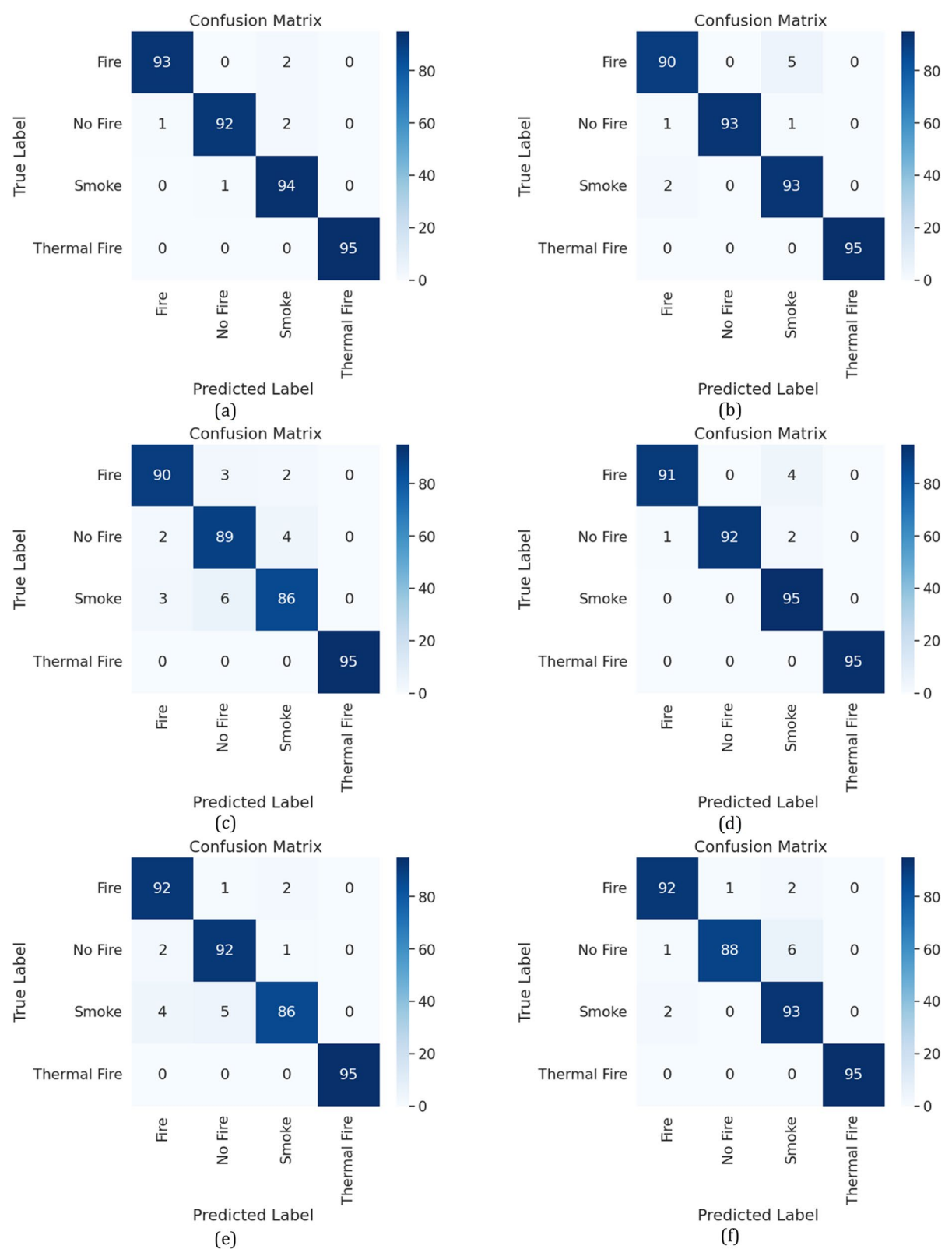
Fig. 7 The confusion matrices of a the proposed FireXnet model, b Densenet201, c VGG16, d MobileNetV2, e InceptionResNetV2, f InceptionV3
