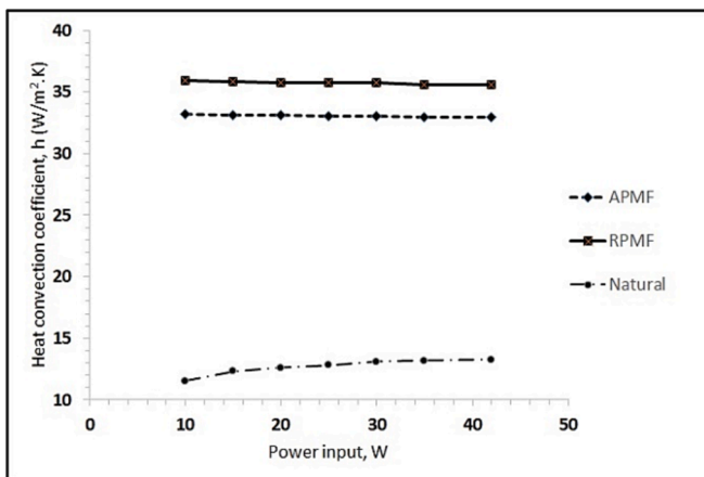
Fig. 11. Comparison of heat convection coefficient for APMF and RPFM.
