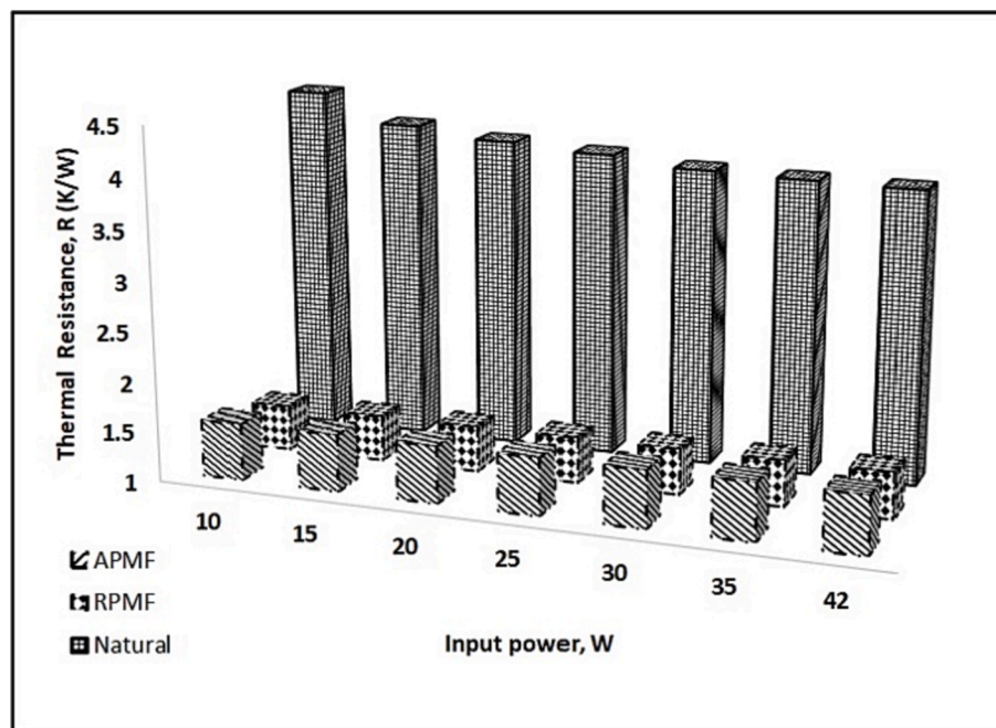
Fig. 9. Comparison of thermal resistance between natural convection, APMF.
