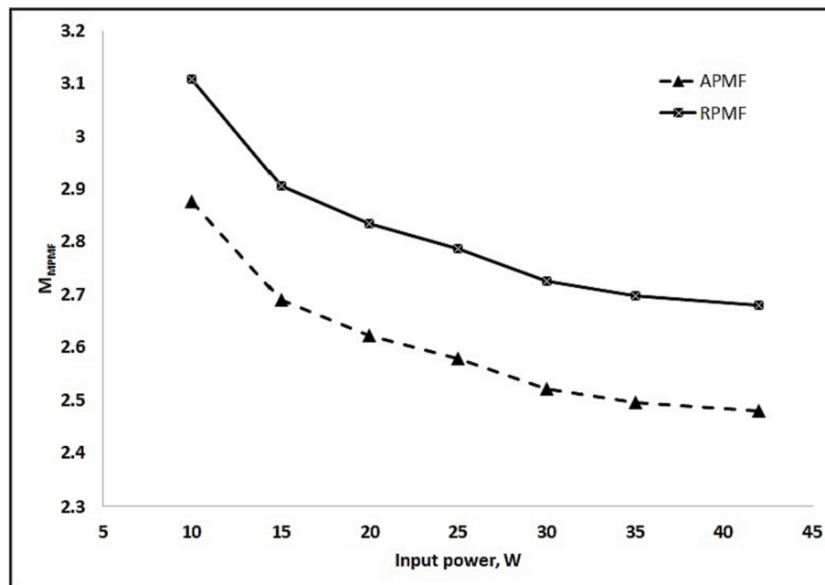
Fig. 12. Comparison of dimensionless coefficient between AMPF and RPFM.
