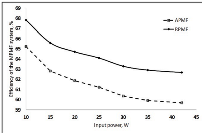
Fig. 10. Comparison of thermal efficiency between APMF and RPFM.
