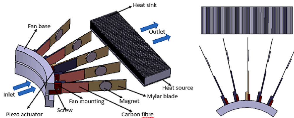
Fig. 1. Schematic diagram of RPFM.
