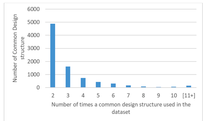
Fig. 8. Reuse frequency of design structures in the valve datasets.
