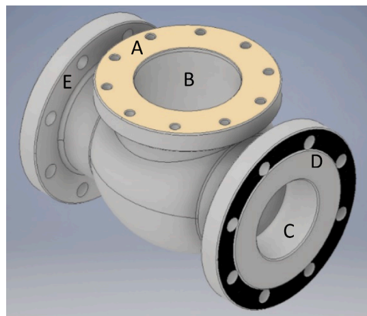
Fig. 1. Patterns of holes in a valve design.
