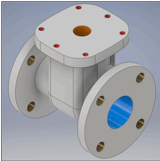
Fig. 13. The chosen four-hole feature valve body used to illustrate the process of identifying substitutable features (CDSs associated with hole features are highlighted in different colours). (For interpretation of the references to colour in this figure legend, the reader is referred to the web version of this article.)
