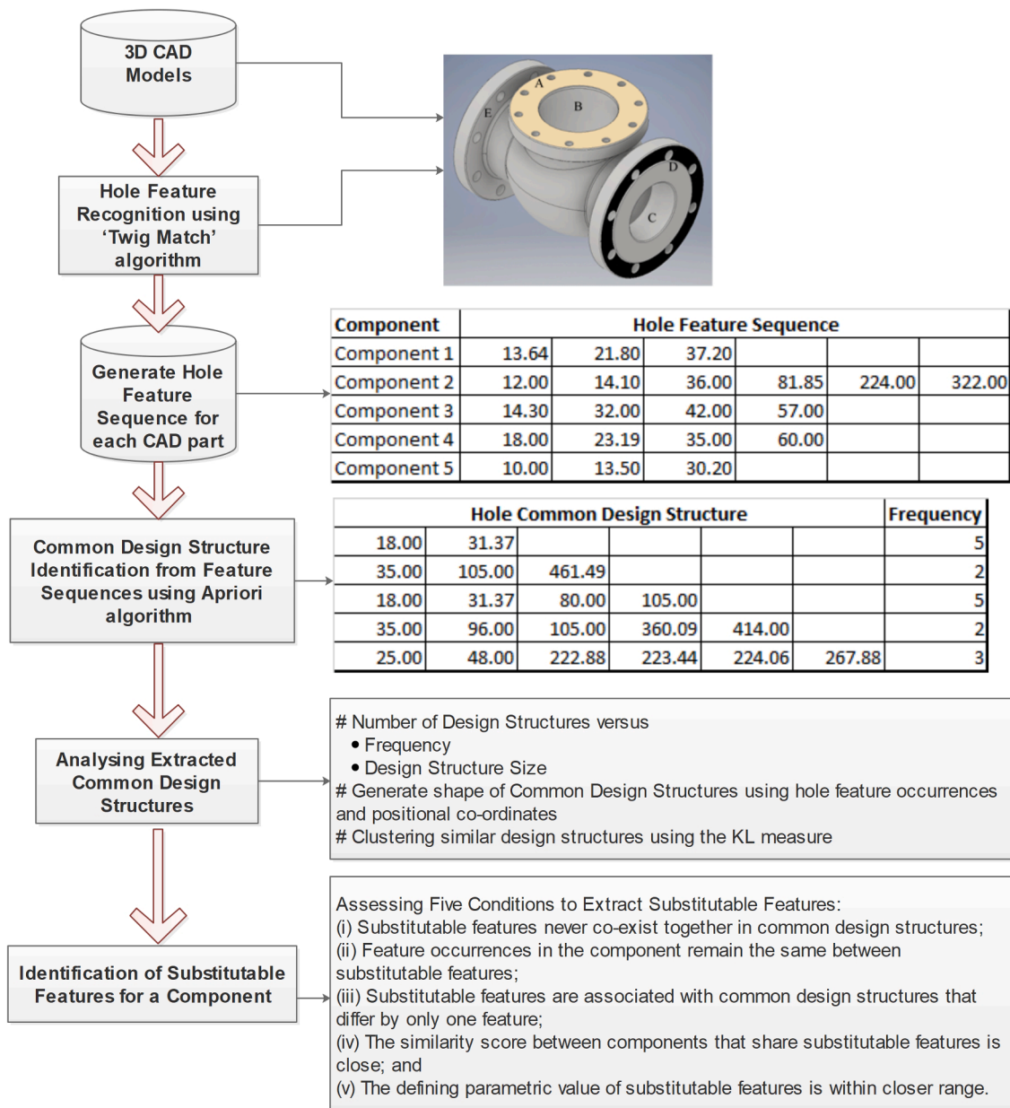
Fig. 2. Process for the discovery of CDS of hole feature and substitutable features.
