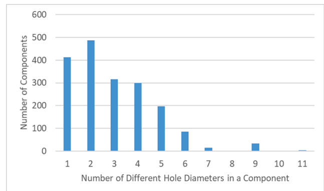
Fig. 4. Frequency of number of different hole diameters in a component.
