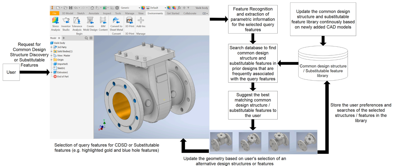
Fig. 15. Schematic illustration of how the common design structure and substitutable feature discovery would function within a feature-based design system.
