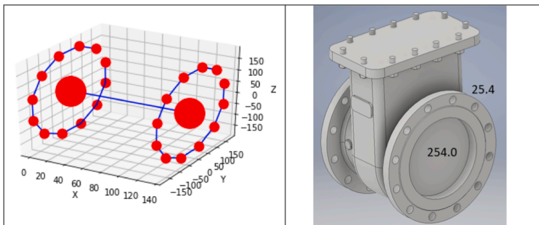
Fig. 3. The shape of a ([25.4, 254.0]) generated hole design structure and its associated 3D component.
