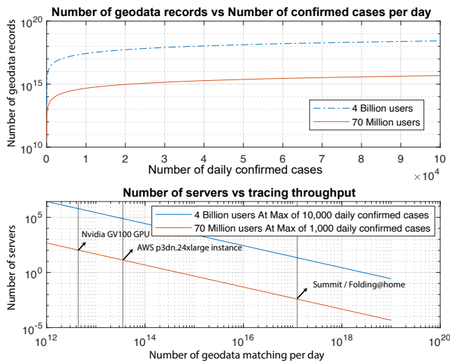
Fig. 4. Computing Resource Requirement for Contact Tracing Geodata matching
