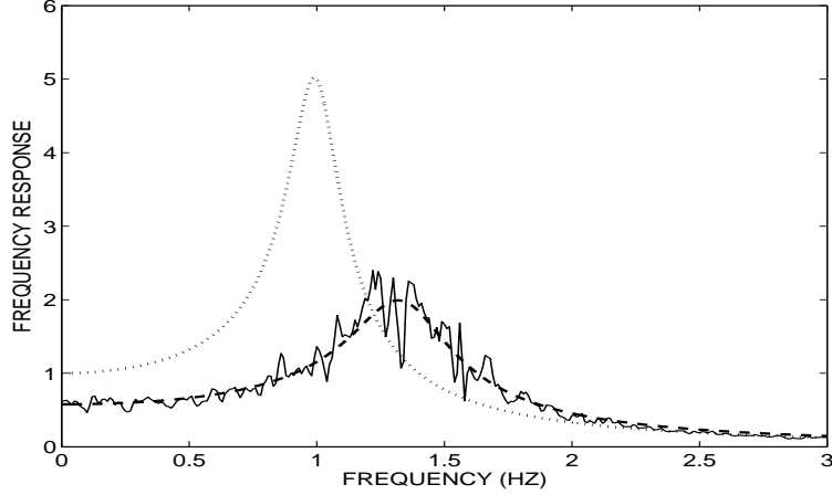
Fig. 2. Frequency response functions for k' = 0.4 and 5% noise using 10 frames to average.
