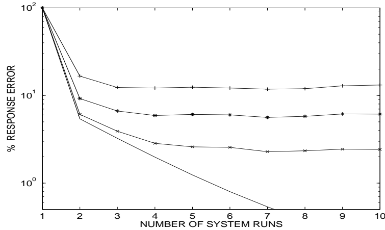
Fig. 11. Results of applying the method using system identification for various levels of noise. The drive used to estimate the non-linearity, k' = 0.4 , is band-limited random noise, employing the full record.
