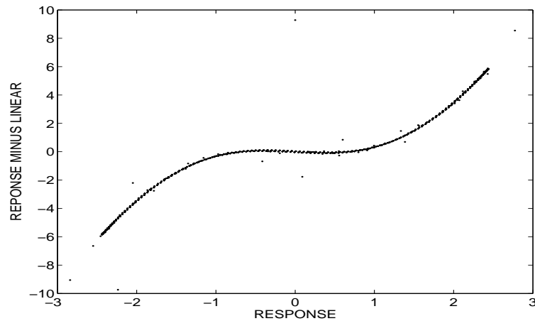
Fig. 6. Estimation of non-linearity for k' = 0.4 using a sinusoid of amplitude 2.0 and frequency of 1.4Hz with no noise – full record with outliers.
