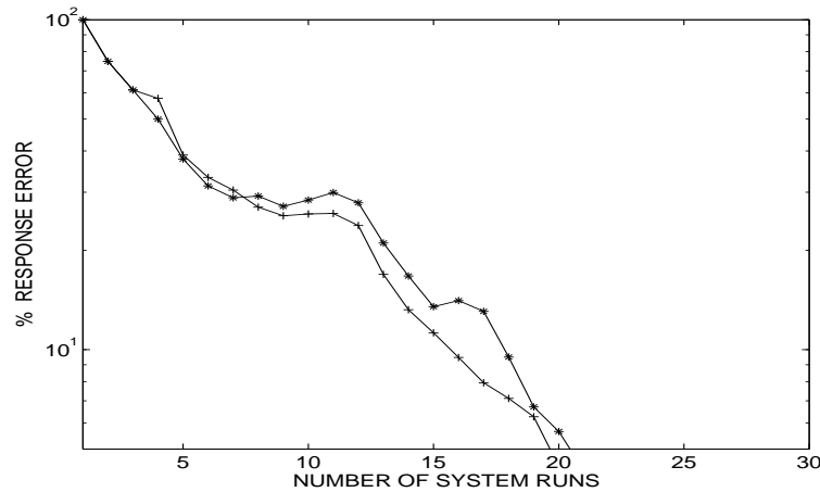
Fig. 3. The fractional error in the response as a function of the number of system runs, both for the conventional (*) and Broyden (+) methods. The nonlinear coefficient is k' = 0.3 . There is no noise and the iteration gain is 0.5.
