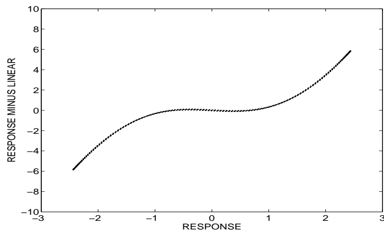
Fig. 7. Estimation of non-linearity for k' = 0.4 using a sinusoid of amplitude 2.0 and frequency of 1.4Hz with no noise – reduced record which removes outliers.
