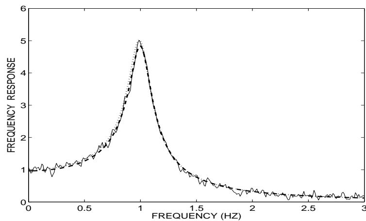
Fig. 5. Plot of the magnitude of frequency response functions for k' = 0.4 and noise of 5%..
