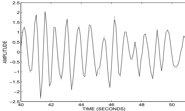
Fig. 12. Part of the desired and achieved response signals using system identification for k' = 0.4 and 10% noise.
