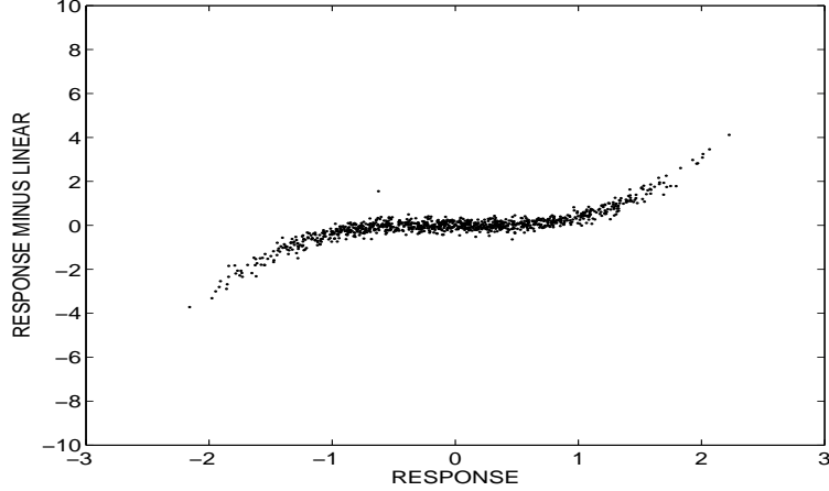
Fig. 8. Estimation of non-linearity for k' = 0.4 and no noise, using a random drive. The cubic nature of the relationship is apparent and a ready estimate of the polynomial may be made using the facilities in MATLAB to perform a least squares fit to produce a vector valued cubic:
