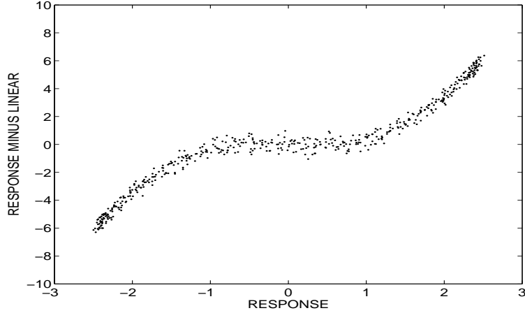
Fig. 10. Plot of (\mathbf{x} - \tilde{\mathbf{C}}\mathbf{y})_i vs \mathbf{y}_i for k' = 0.4 and 5% noise, using a sinusoid of reduced record.
