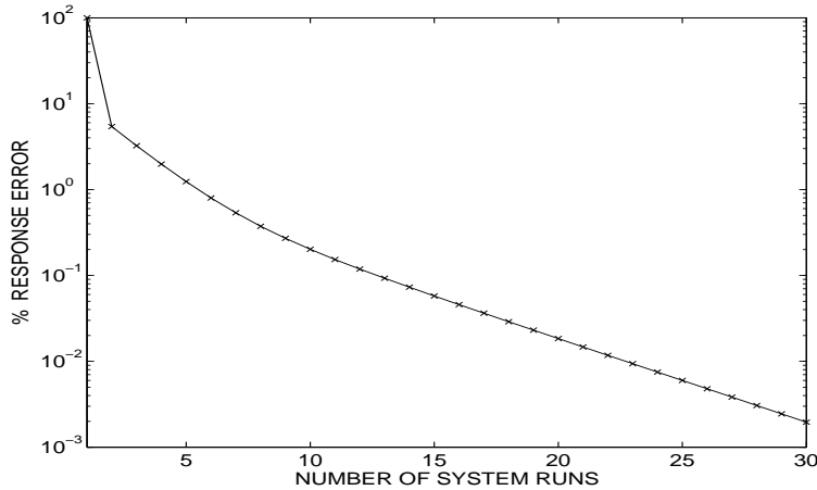
Fig. 9. Fractional error in response using system identification for k' = 0.4 and no measurement noise. The drive used to estimate the nonlinearity is bandlimited white noise.
