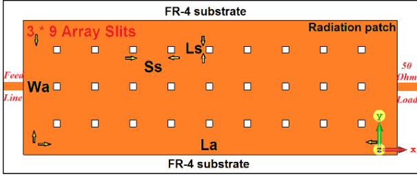
(a) Top view of the leaky-wave antenna
