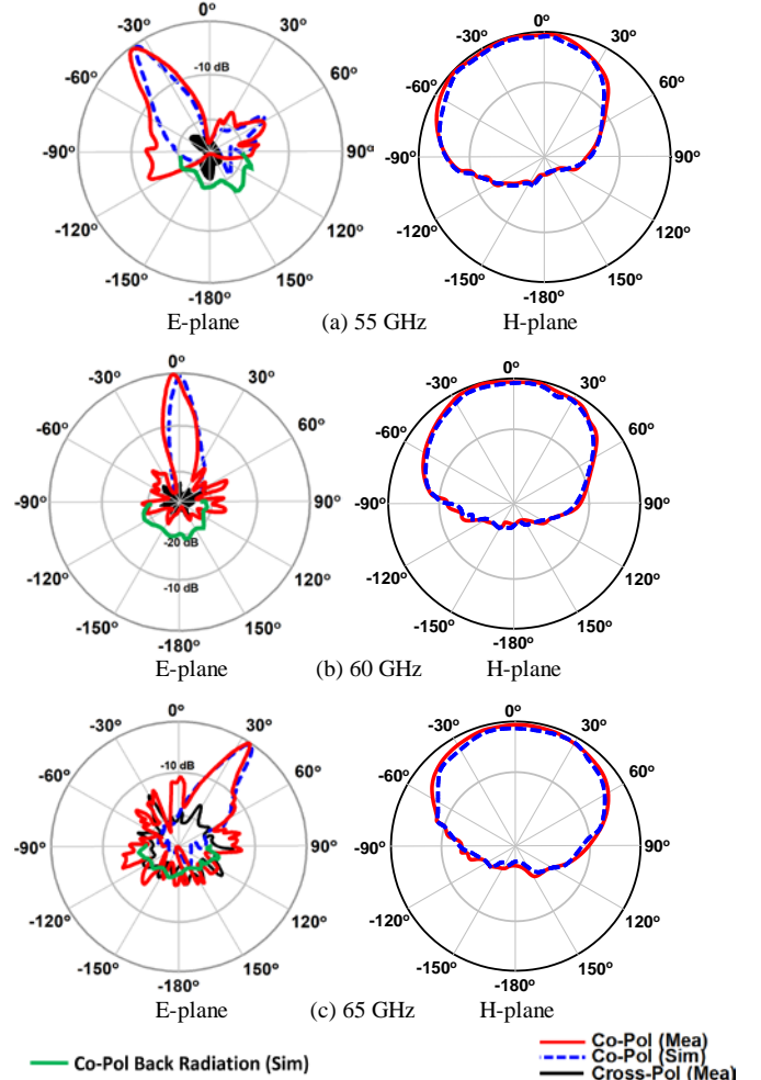
Fig. 9. Simulated and measured E-plane ( xz -plane) and H-plane ( yz -plane) backward to forward radiation patterns of the proposed beam-steering antenna at (a) 55 GHz, (b) 60 GHz, and (c) 65 GHz.
