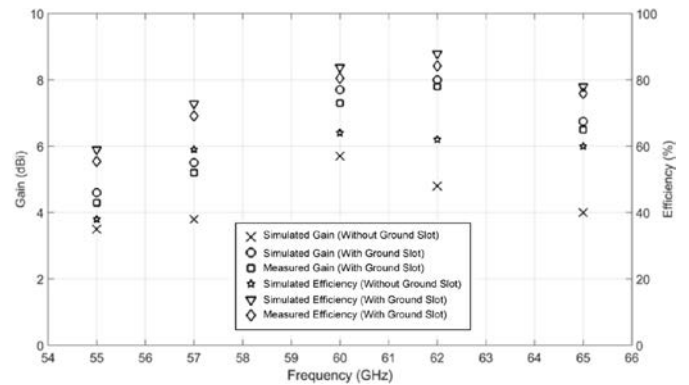
Fig. 7. Gain and radiation efficiency response of the proposed LWA when it's unloaded and loaded with ground-plane slots.
