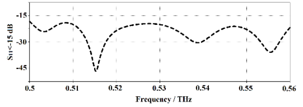
Fig.2. Frequency bandwidth ( S_{11} < -15\text{dB} ) of the on-chip antenna.
