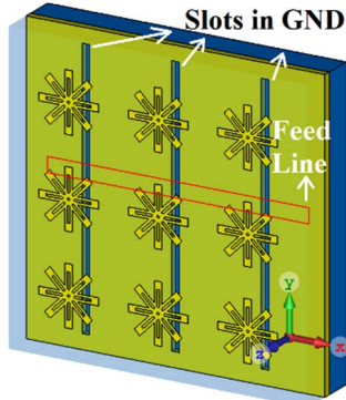
(b) Isometric view showing asterisk-shaped elements on the top silicon layer, slot-lines in the ground-plane layer, and open-ended microstrip feed line on the bottom silicon layer.
