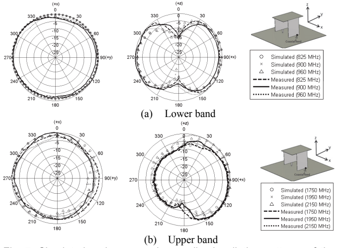
Fig. 7. Simulated and measured normalized radiation patterns of the proposed antenna.
