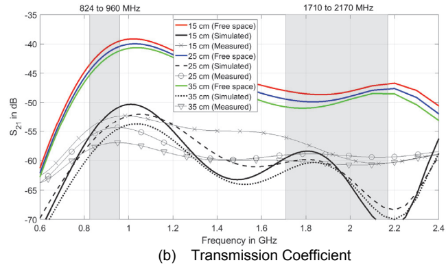
Fig. 13. S-parameters between the horn antenna and the antenna under test (AUT) at different depths in the manhole chamber.
