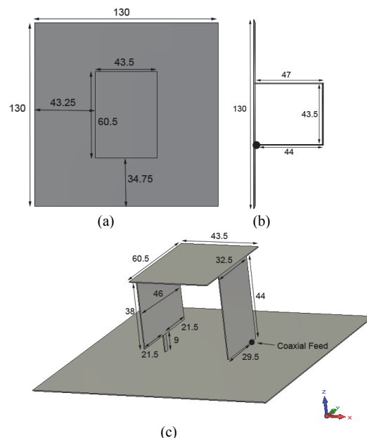
Fig. 1. Geometry of the proposed antenna (Units: mm). (a) Top view, (b) Side view, (c) Auxiliary view.
