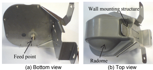
Fig. 14. Antenna prototype for field trial.
