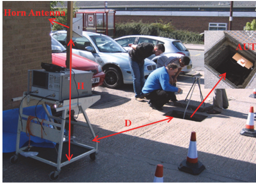
Fig. 12. On-site measurement setup.
