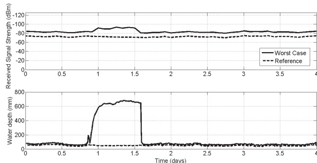
Fig. 15. Received signal strength level of transceiver versus the water depth in the manhole chamber in a practical site over a worst-case time period.
