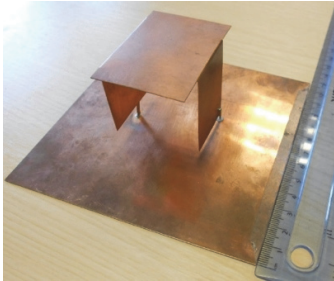
Fig. 5. Prototype of the proposed antenna.
