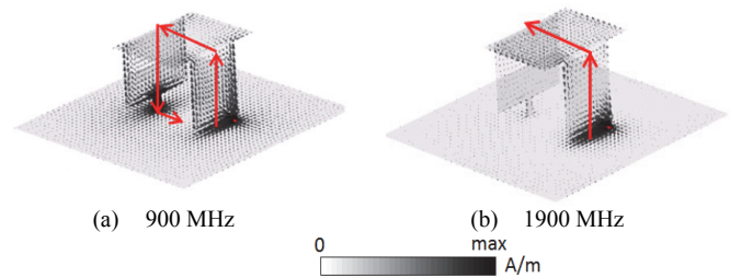
Fig. 4. Current distributions of the proposed antenna.
