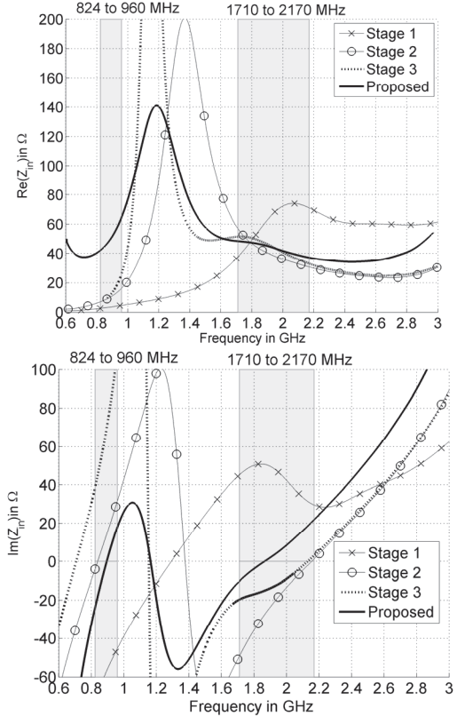
Fig. 3. Simulated input impedance of proposed antenna in the design evolution process as depicted in Fig. 2.
