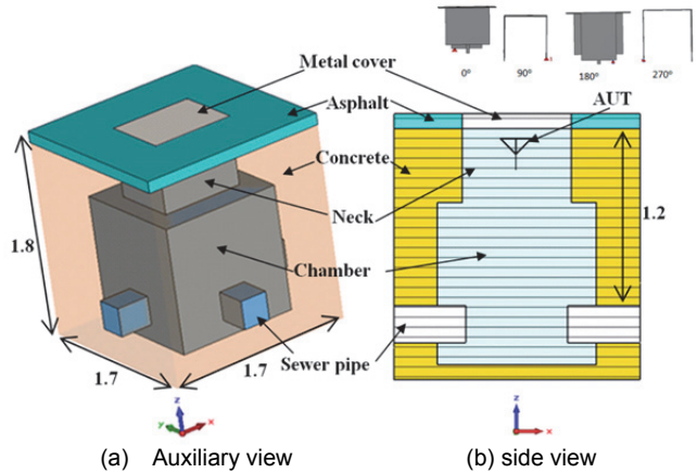
Fig. 8. Antenna in manhole chamber model (Unit: meters).
